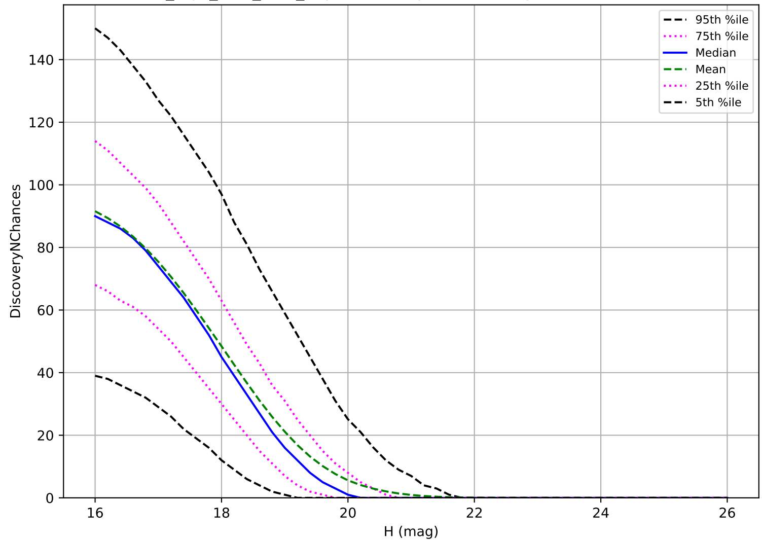
no_high_blob_v3.3_10yrs: MBA 3 pairs in 15 nights detection loss
