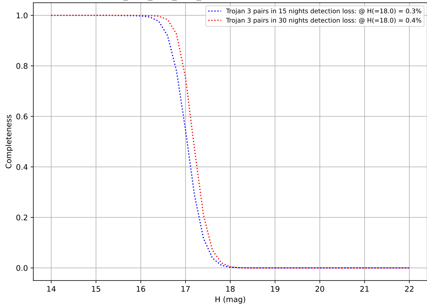
no_high_blob_v3.3_10yrs: DifferentialCompleteness
