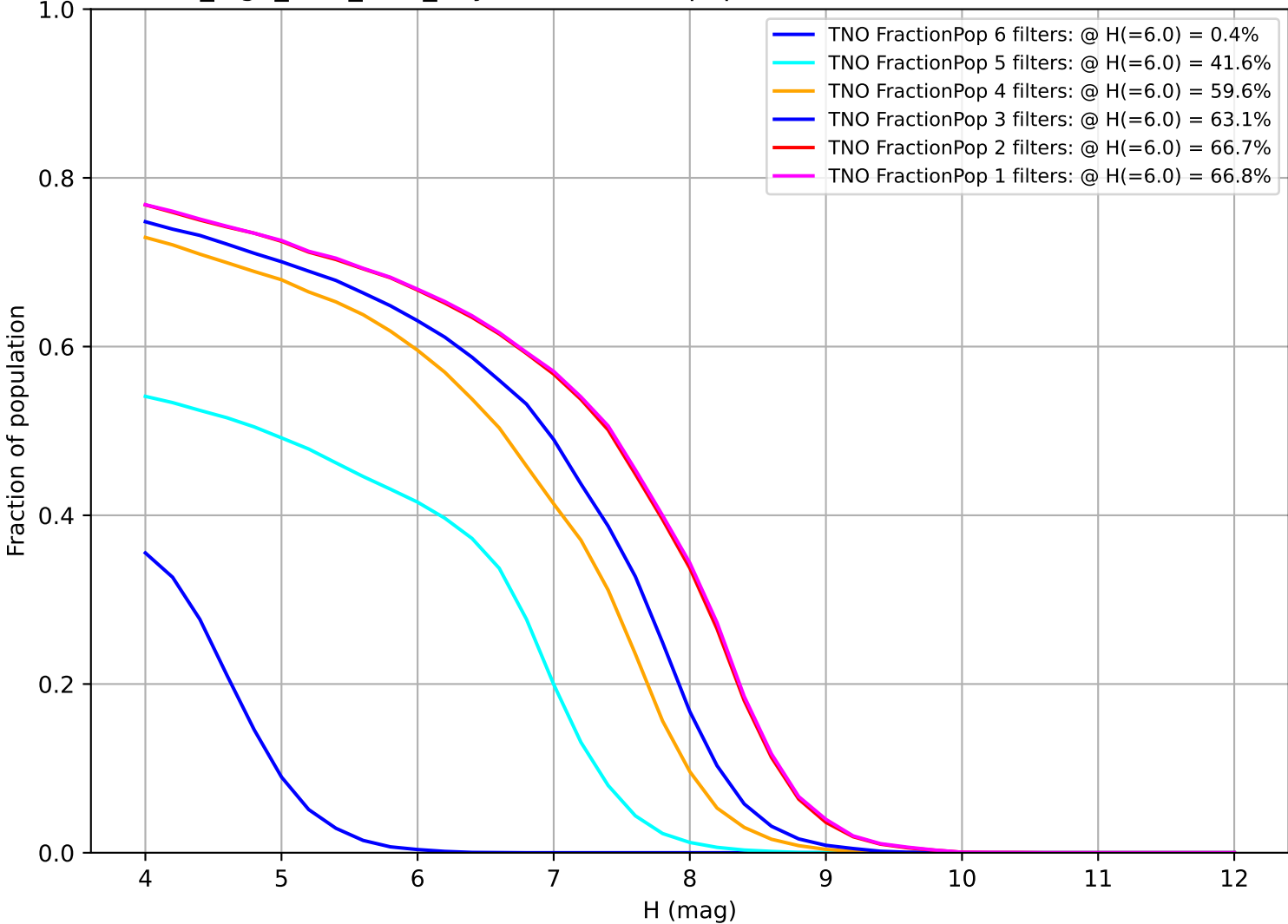
no_high_blob_v3.3_10yrs: Fraction of population with colors in X filters TNO
