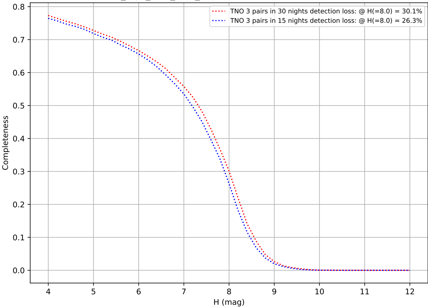
no_high_blob_v3.3_10yrs: DifferentialCompleteness
