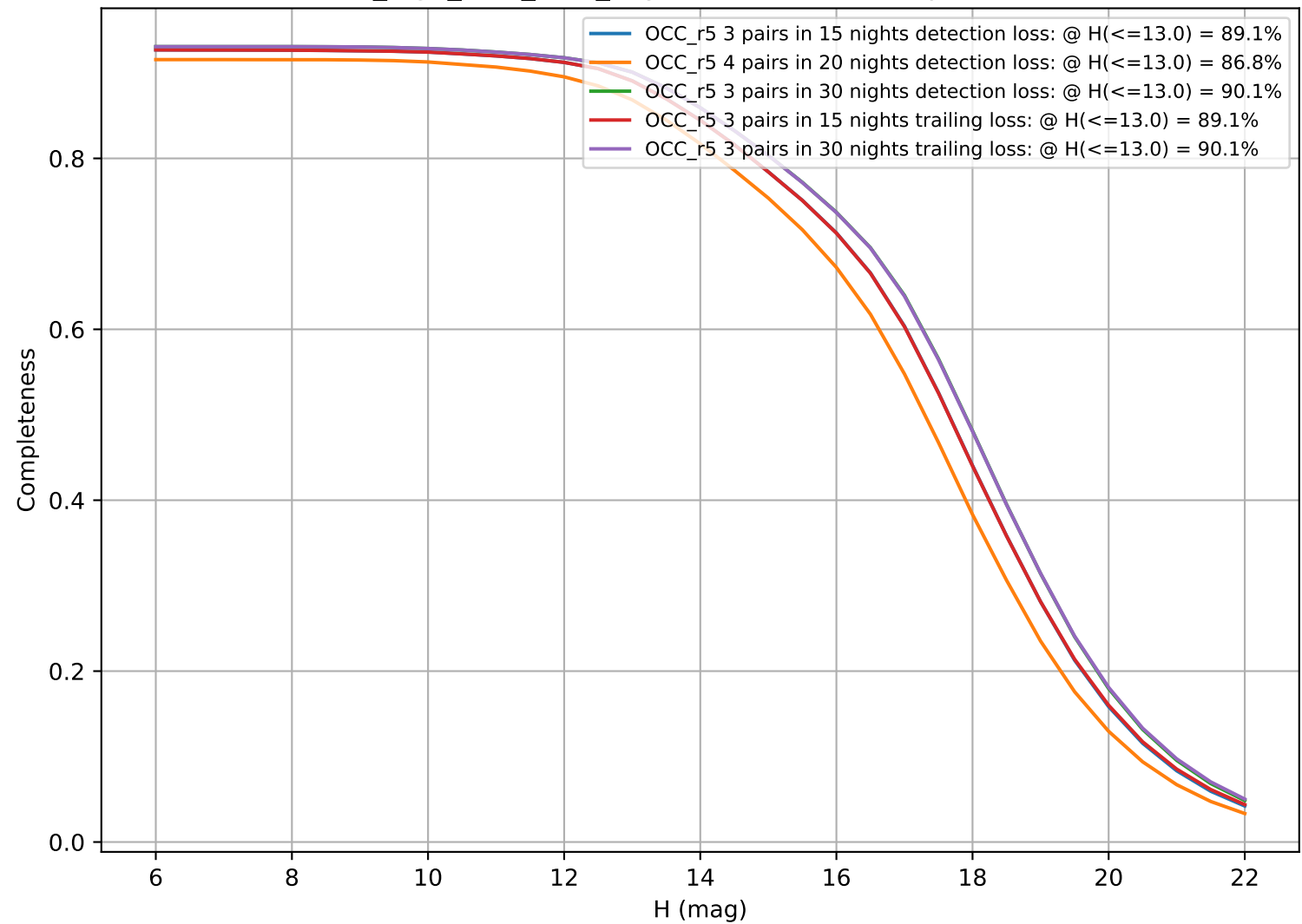
no_high_blob_v3.3_10yrs: CumulativeCompleteness
