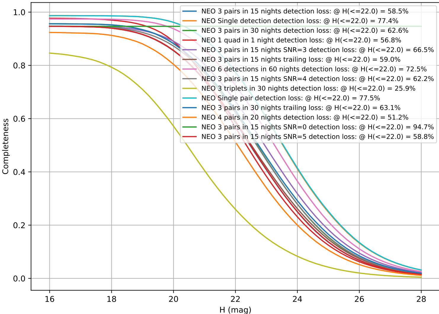
no_high_blob_v3.3_10yrs: CumulativeCompleteness
