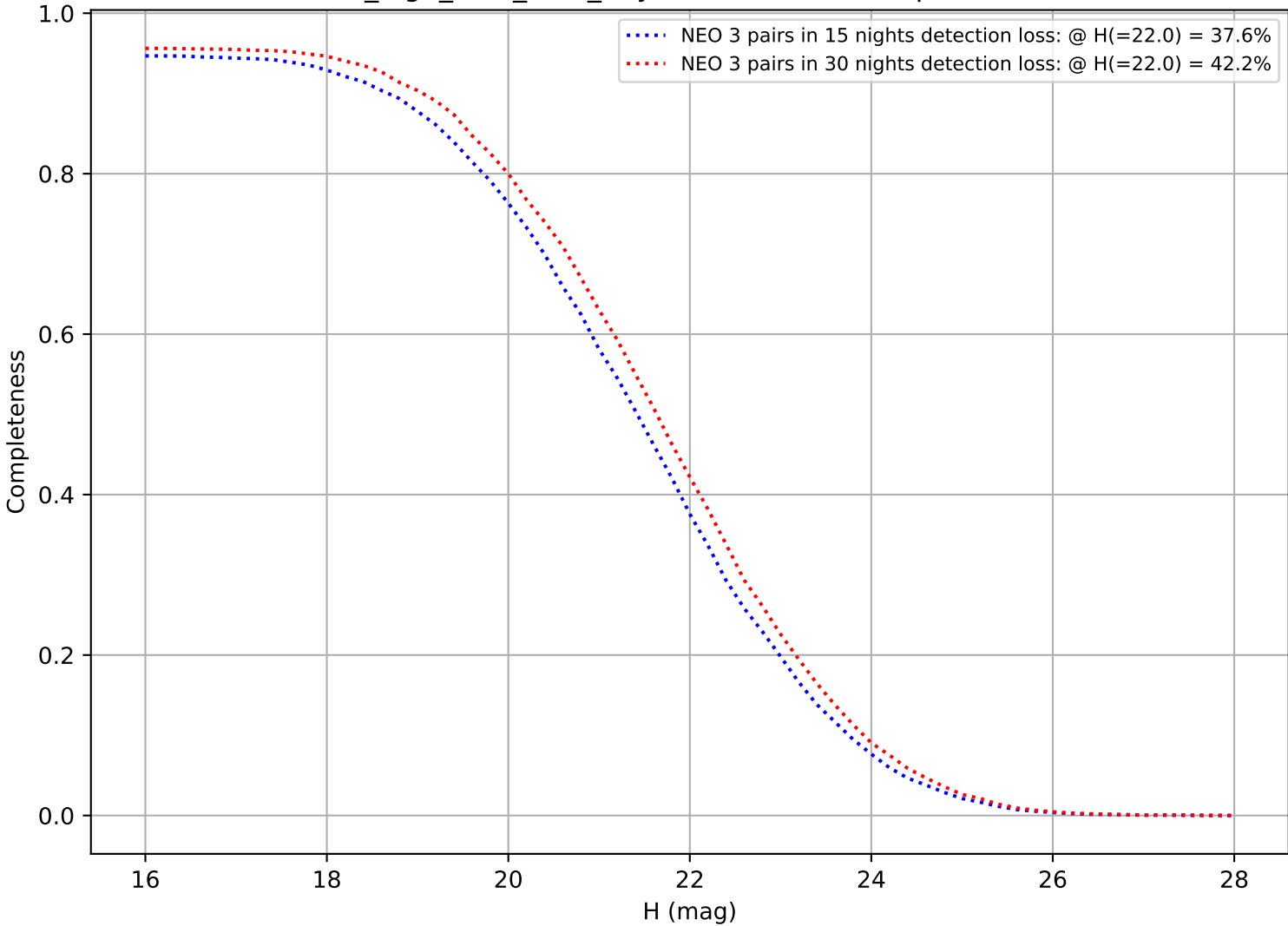
no_high_blob_v3.3_10yrs: DifferentialCompleteness
