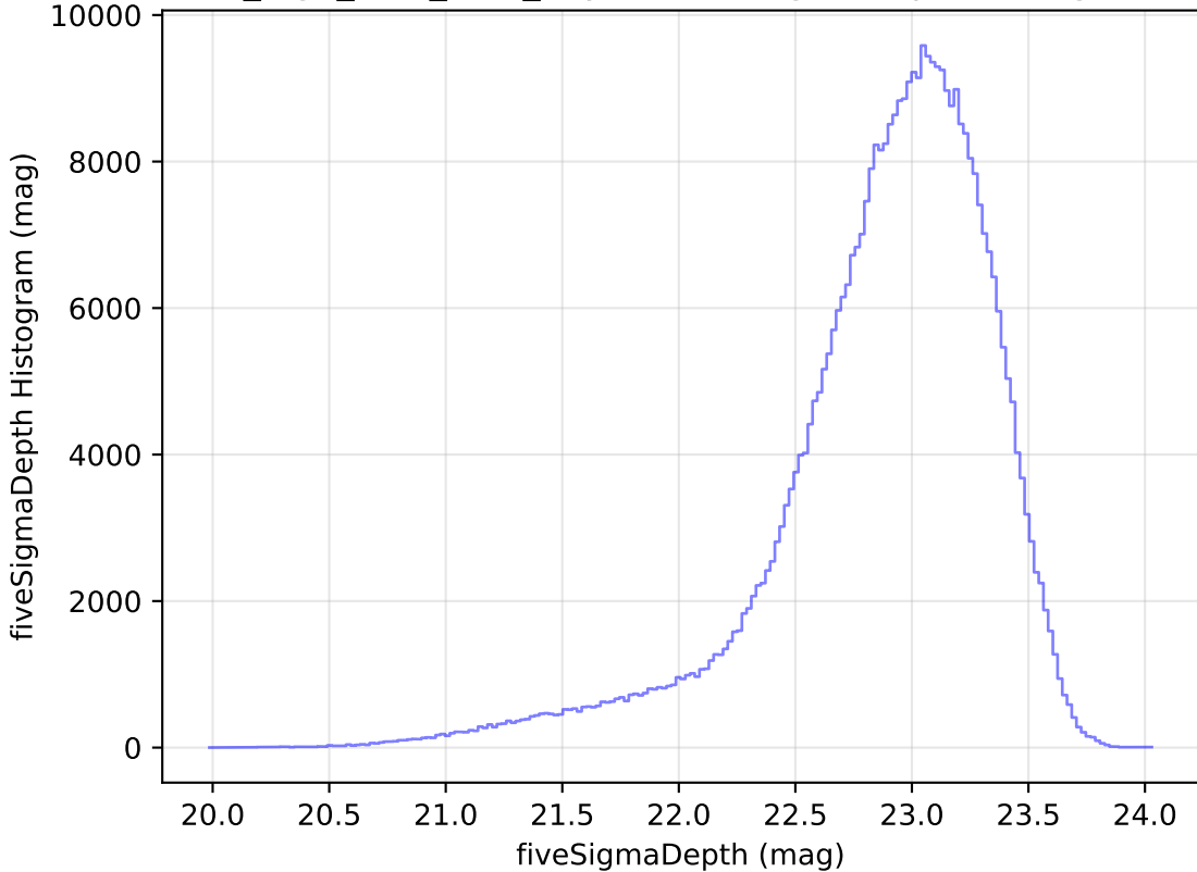
no_high_blob_v3.3_10yrs z: fiveSigmaDepth Histogram
