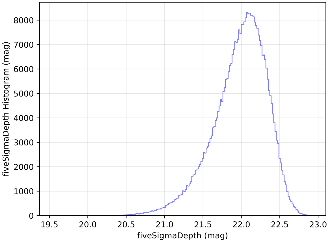
no_high_blob_v3.3_10yrs y: fiveSigmaDepth Histogram
