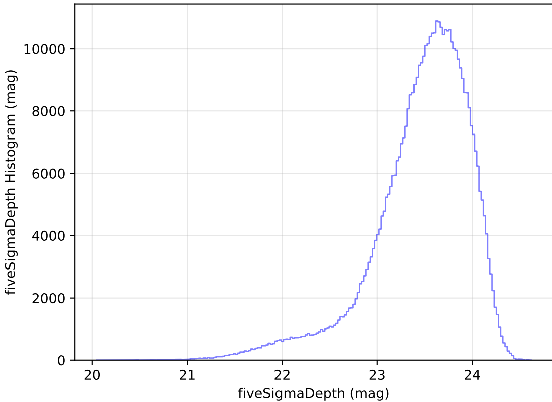
no_high_blob_v3.3_10yrs i: fiveSigmaDepth Histogram
