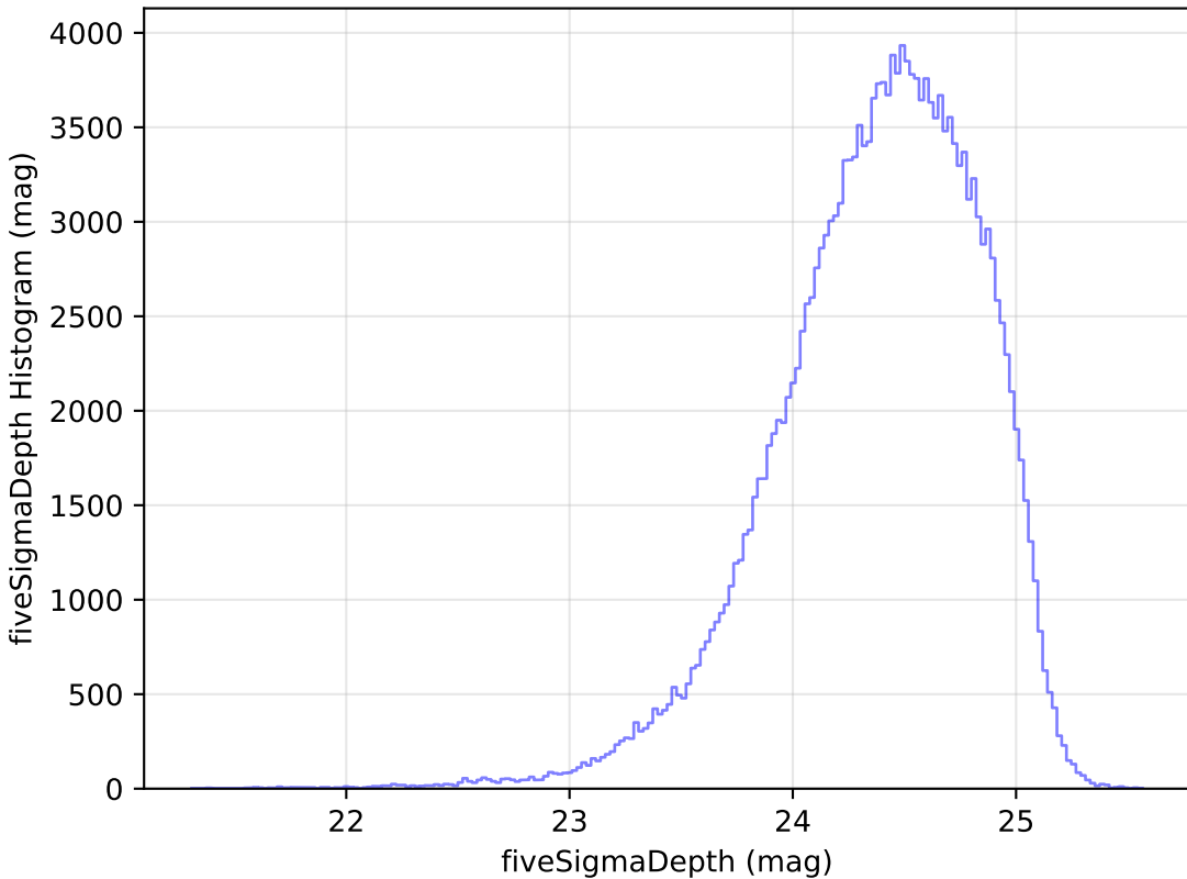
no_high_blob_v3.3_10yrs g: fiveSigmaDepth Histogram
