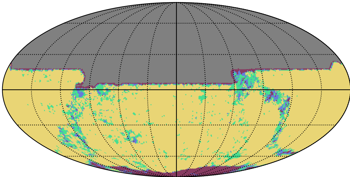
no_high_blob_v3.3_10yrs y band: YearCoverage night
