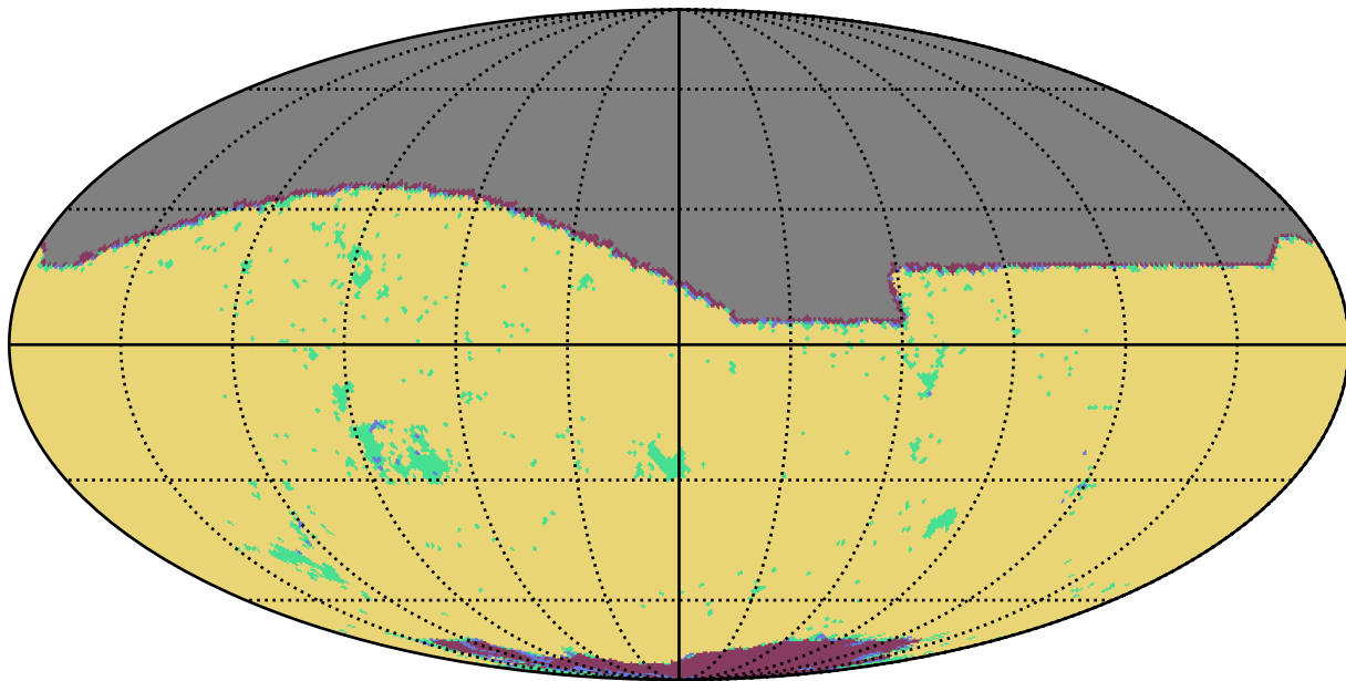
no_high_blob_v3.3_10yrs r band: YearCoverage night
