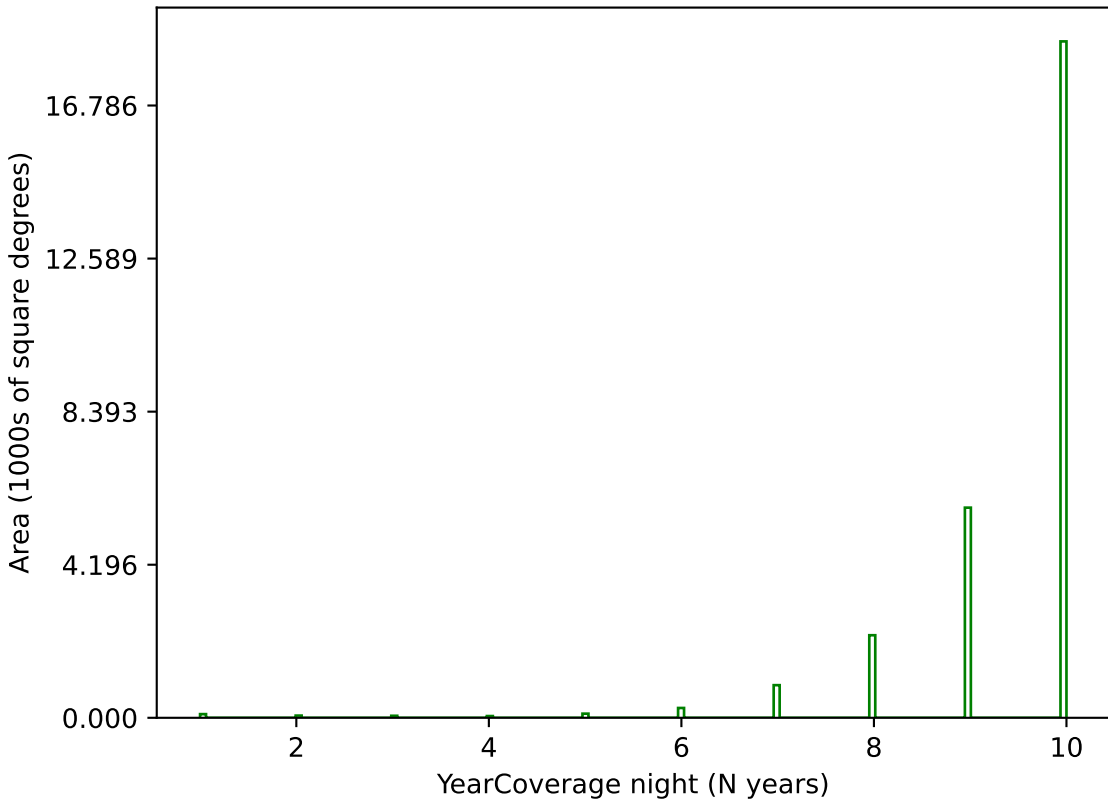
no_high_blob_v3.3_10yrs g band: YearCoverage night
