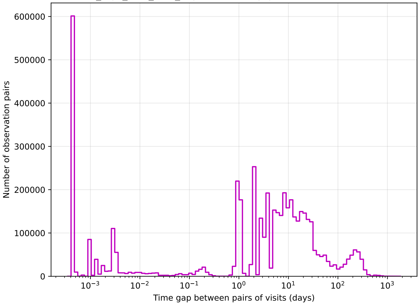
no_high_blob_v3.3_10yrs z band: Tgaps observationStartMJD
