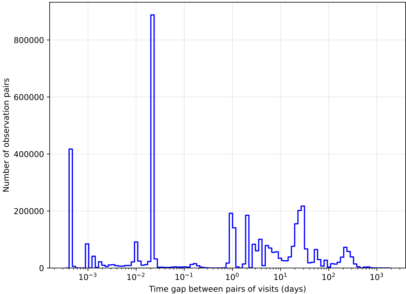
no_high_blob_v3.3_10yrs y band: Tgaps observationStartMJD
