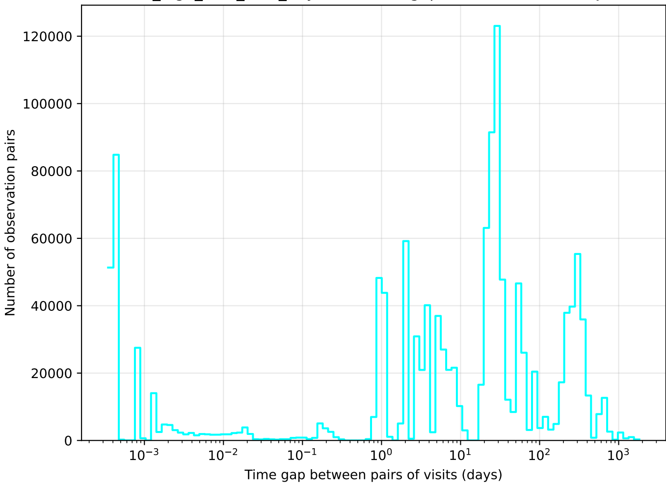
no_high_blob_v3.3_10yrs u band: Tgaps observationStartMJD
