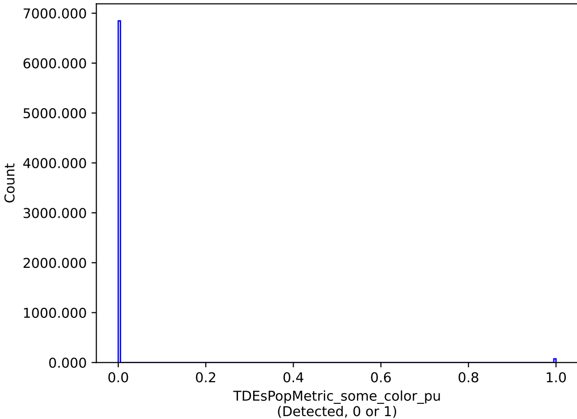
no_high_blob_v3.3_10yrs : TDEsPopMetric_some_color_pu
