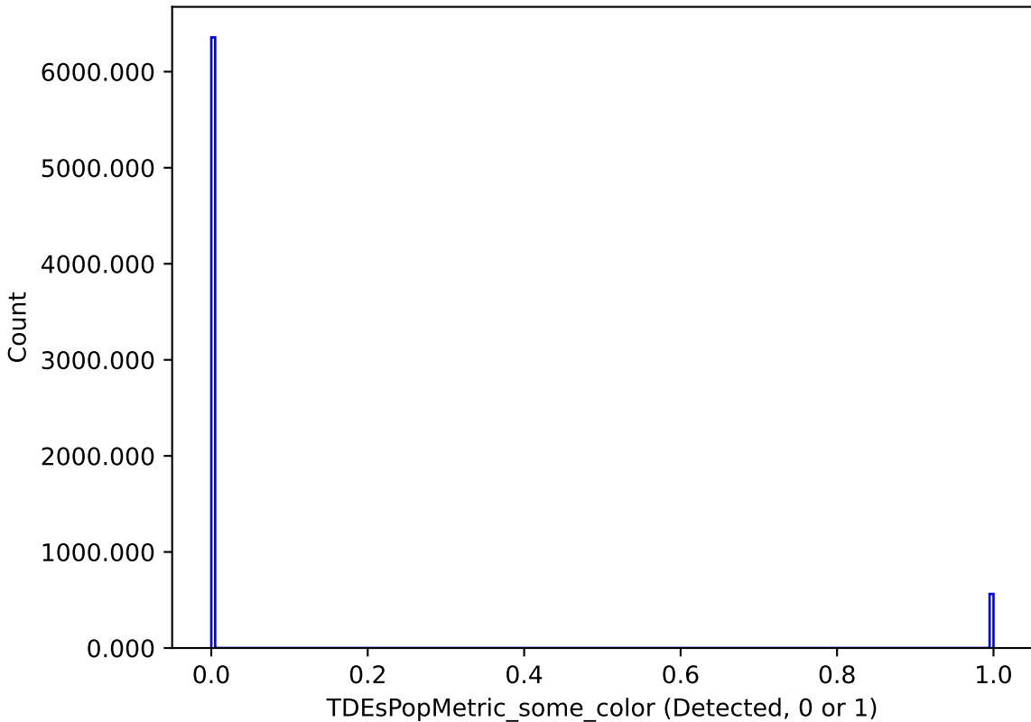
no_high_blob_v3.3_10yrs : TDEsPopMetric_some_color
