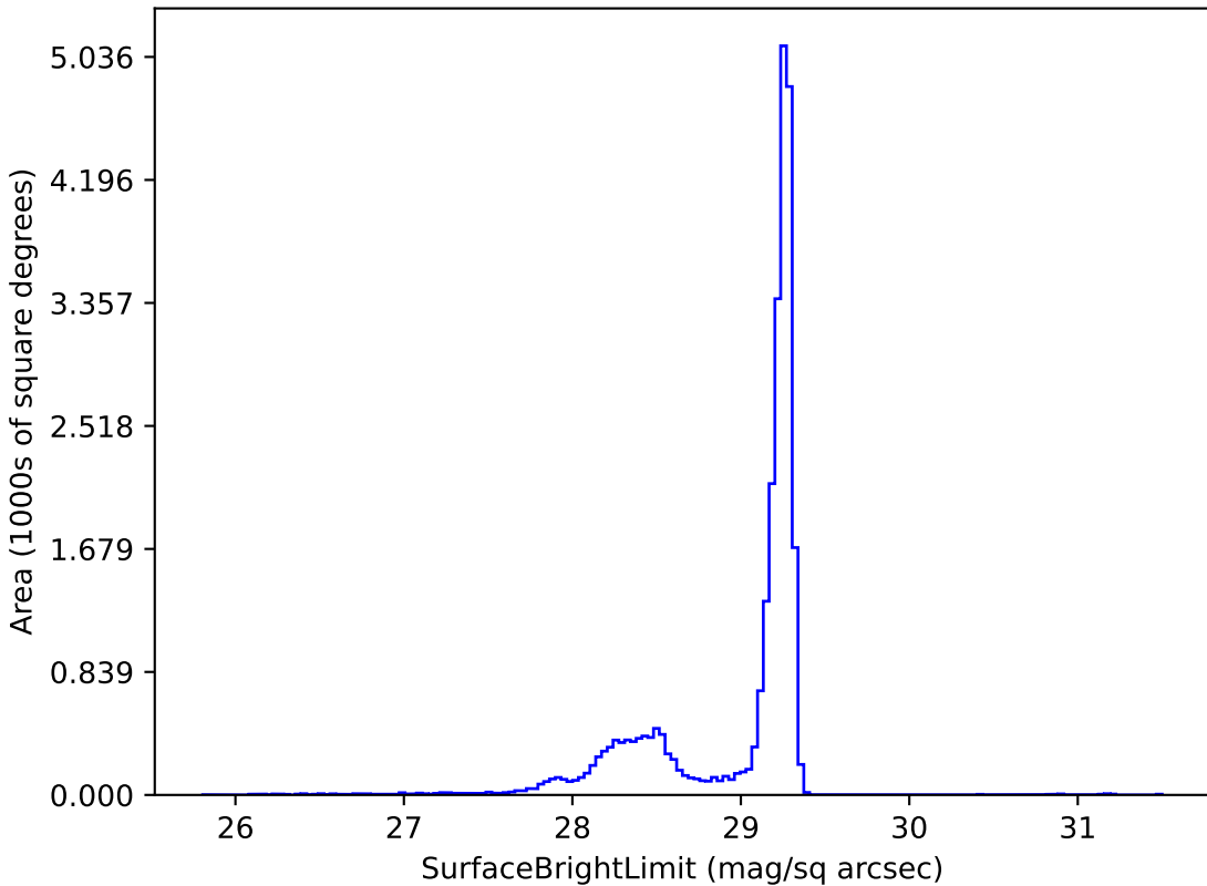
no_high_blob_v3.3_10yrs z: SurfaceBrightLimit
