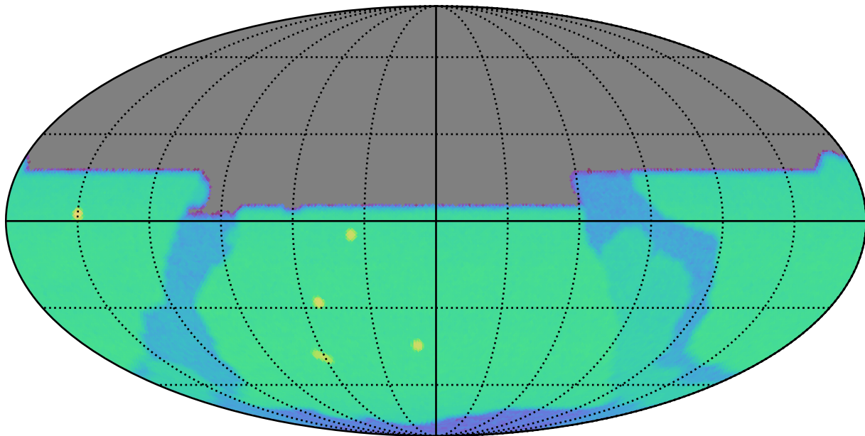
no_high_blob_v3.3_10yrs y: SurfaceBrightLimit
