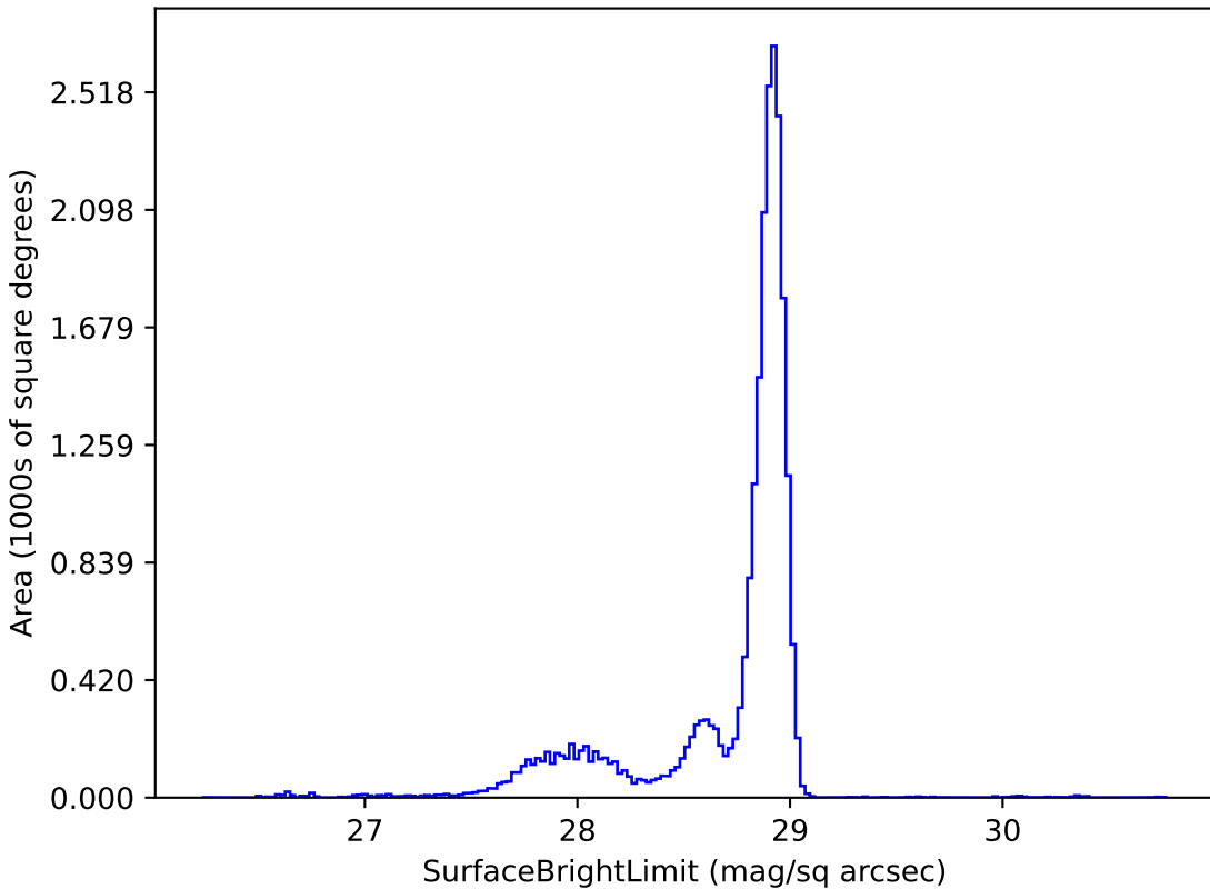
no_high_blob_v3.3_10yrs u: SurfaceBrightLimit
