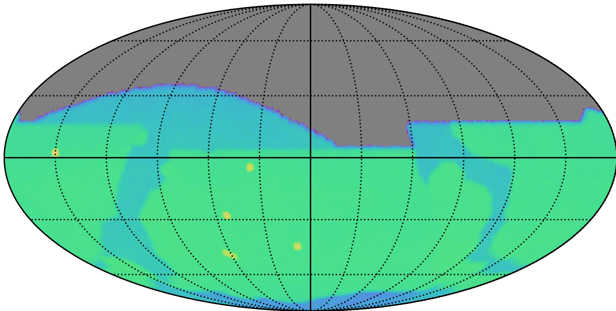
no_high_blob_v3.3_10yrs r: SurfaceBrightLimit
