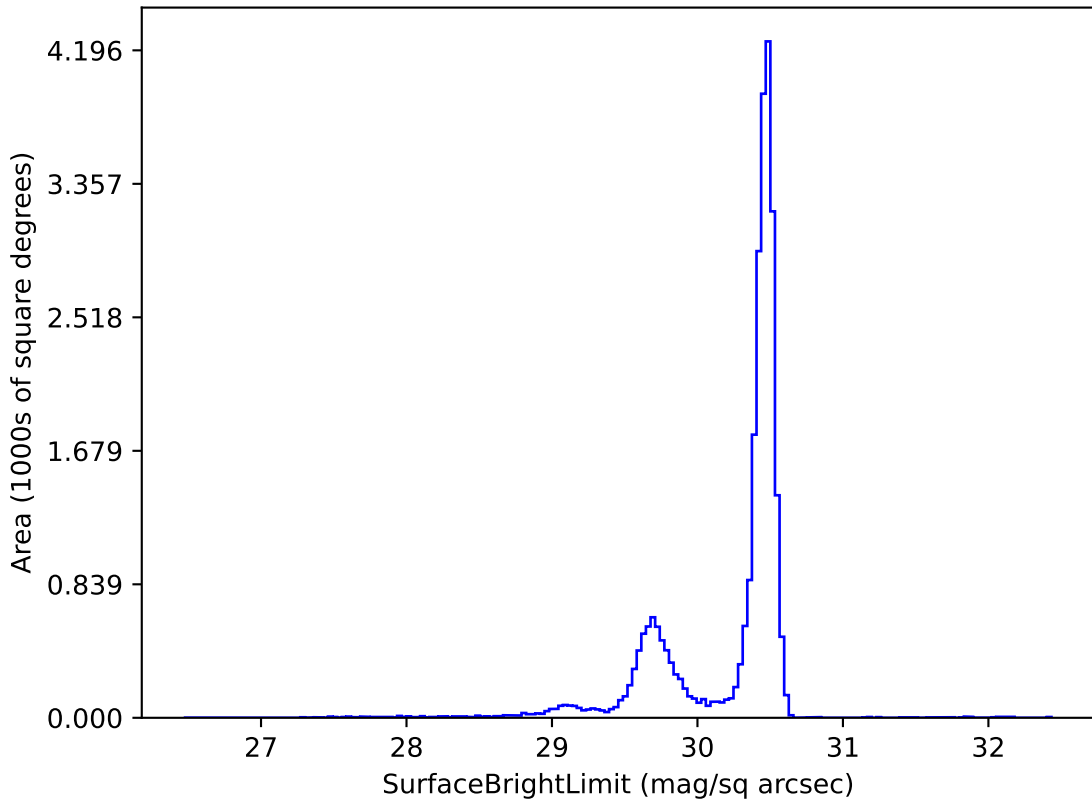
no_high_blob_v3.3_10yrs r: SurfaceBrightLimit
