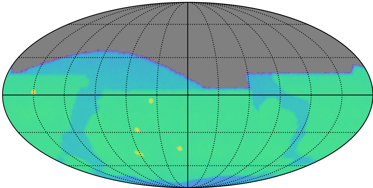
no_high_blob_v3.3_10yrs i: SurfaceBrightLimit
