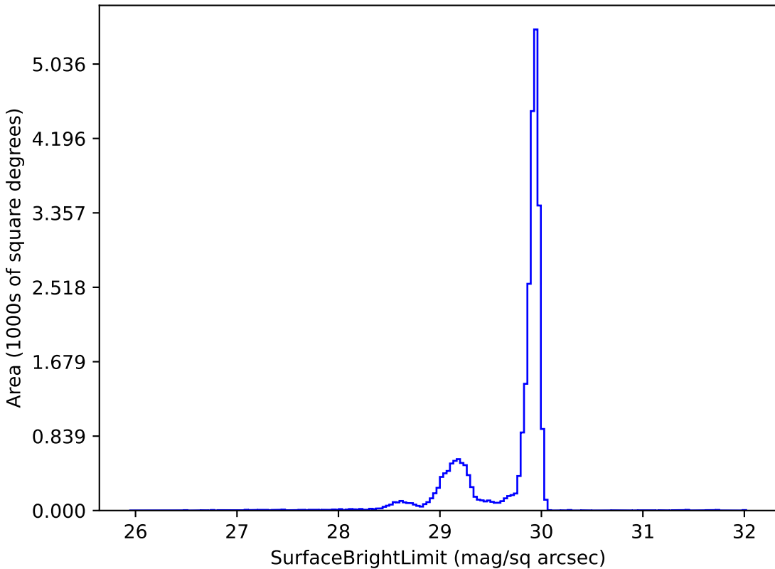
no_high_blob_v3.3_10yrs i: SurfaceBrightLimit
