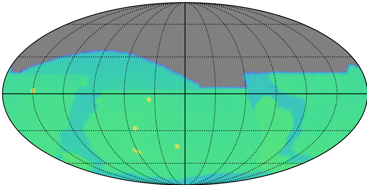
no_high_blob_v3.3_10yrs g: SurfaceBrightLimit
