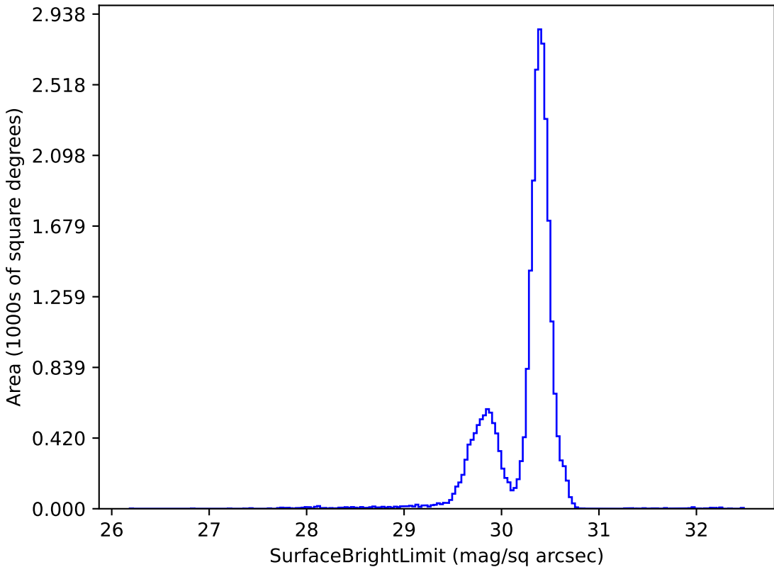
no_high_blob_v3.3_10yrs g: SurfaceBrightLimit
