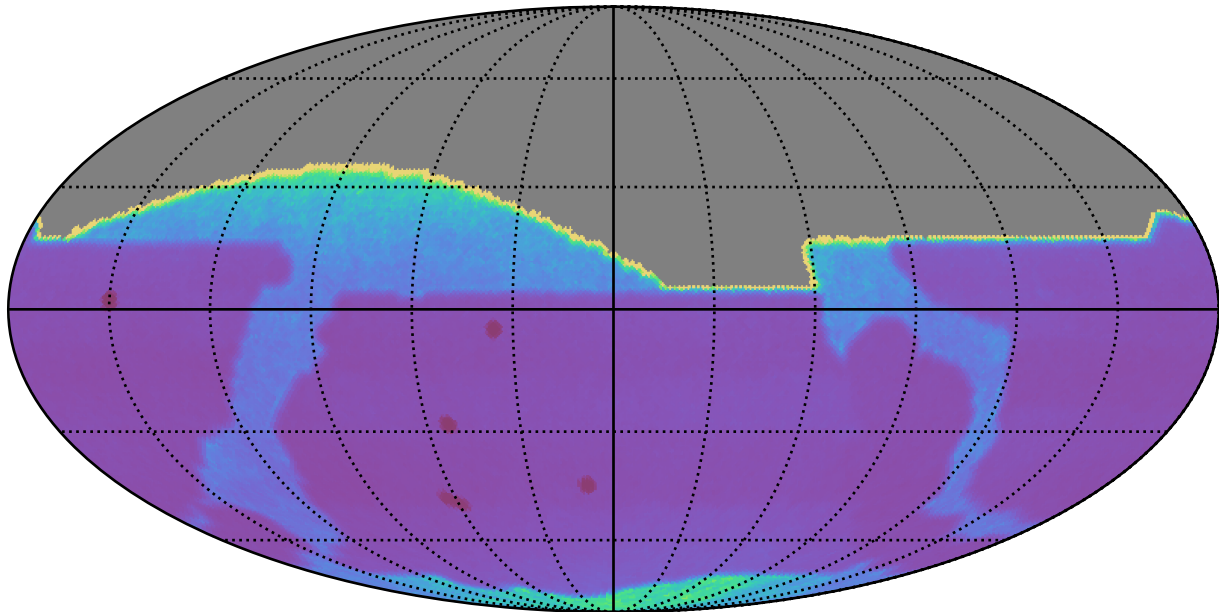
no_high_blob_v3.3_10yrs : Proper Motion Uncert @ 20.5
