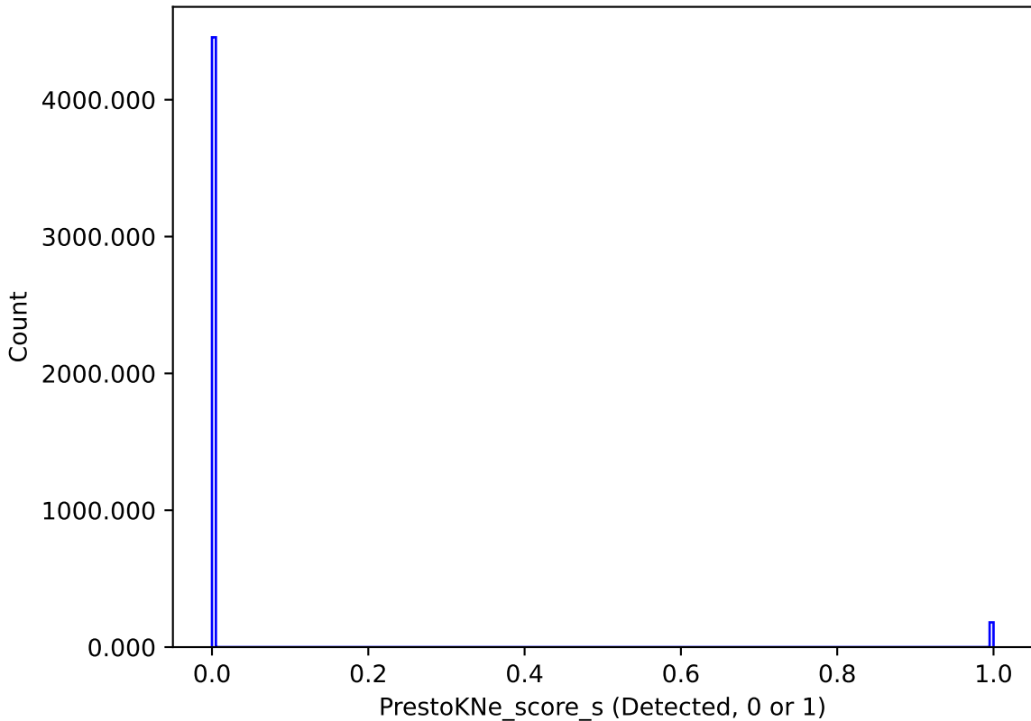
no_high_blob_v3.3_10yrs : PrestoKNe_score_s
