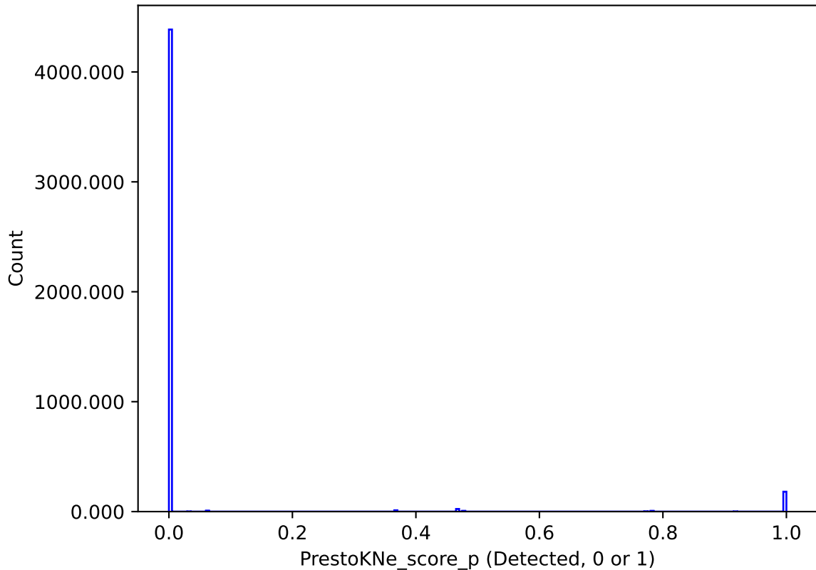
no_high_blob_v3.3_10yrs : PrestoKNe_score_p
