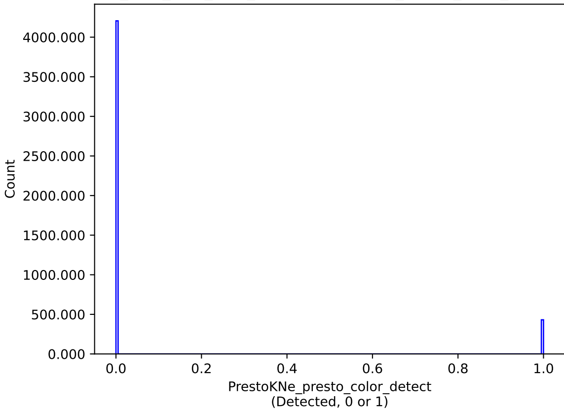
no_high_blob_v3.3_10yrs : PrestoKNe_presto_color_detect
