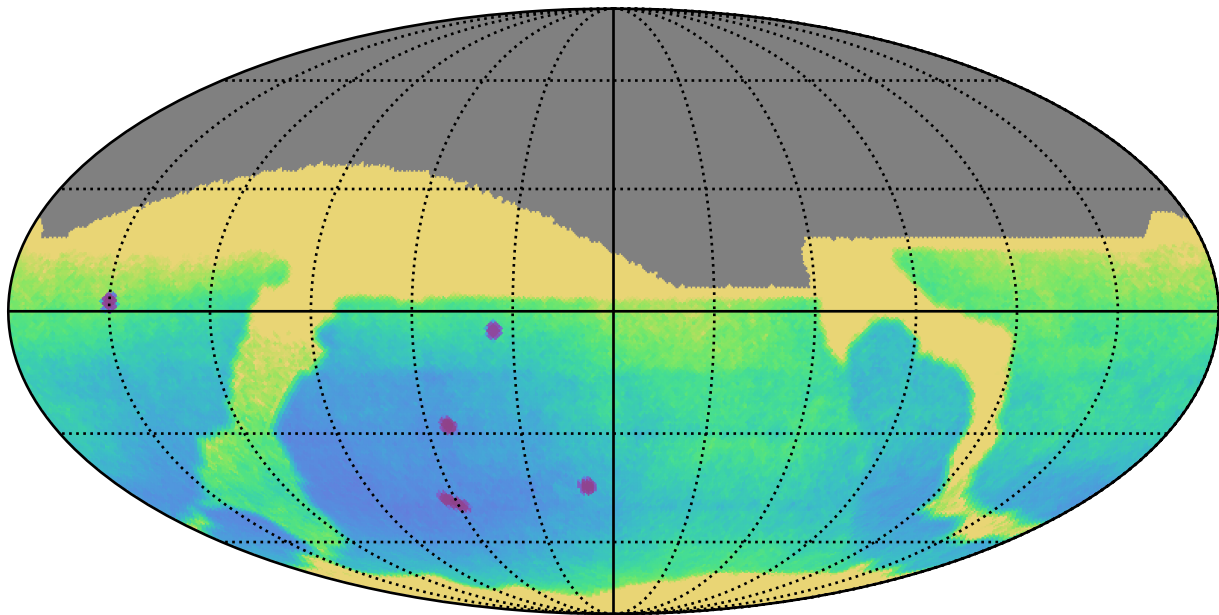
no_high_blob_v3.3_10yrs : Parallax Uncert @ 24.0
