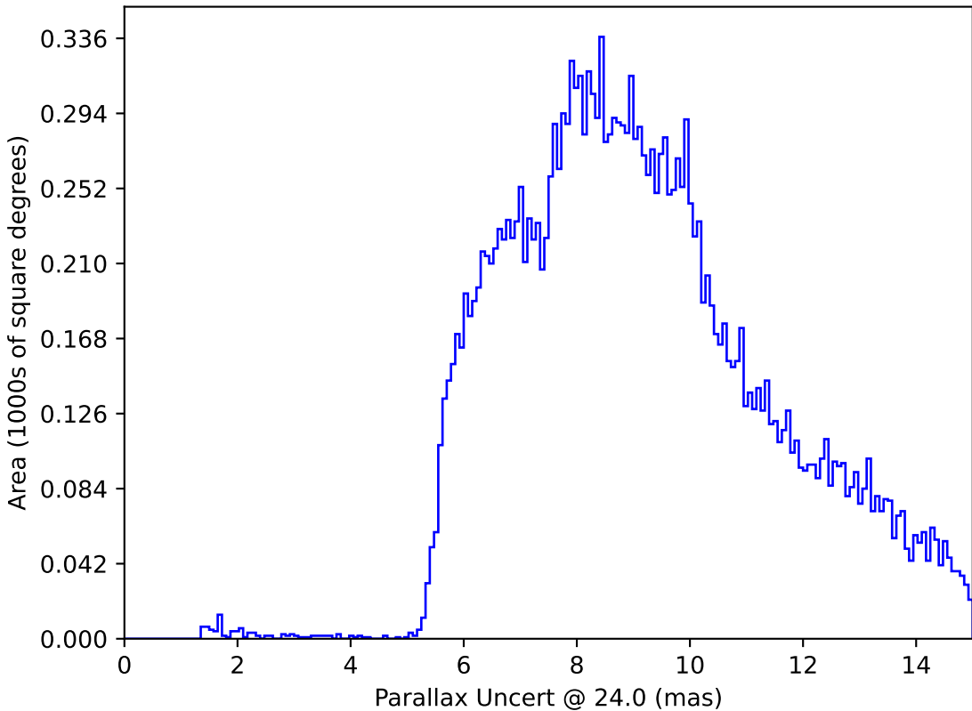
no_high_blob_v3.3_10yrs : Parallax Uncert @ 24.0
