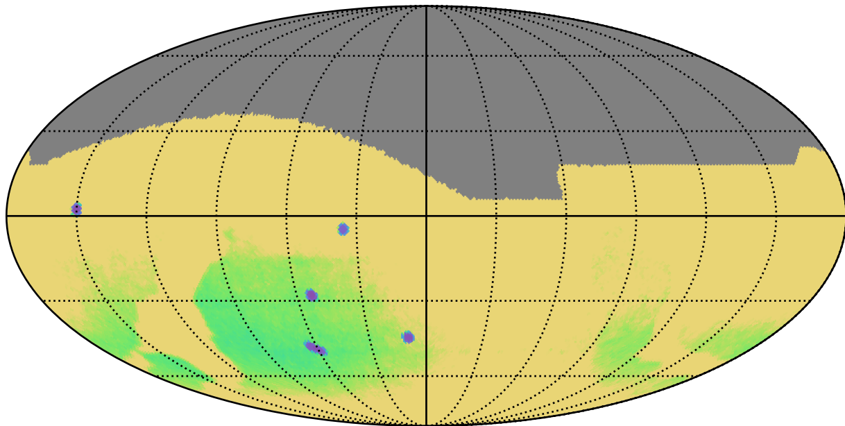
no_high_blob_v3.3_10yrs : Parallax Uncert @ 22.4
