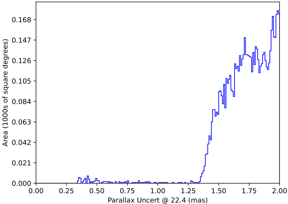
no_high_blob_v3.3_10yrs : Parallax Uncert @ 22.4
