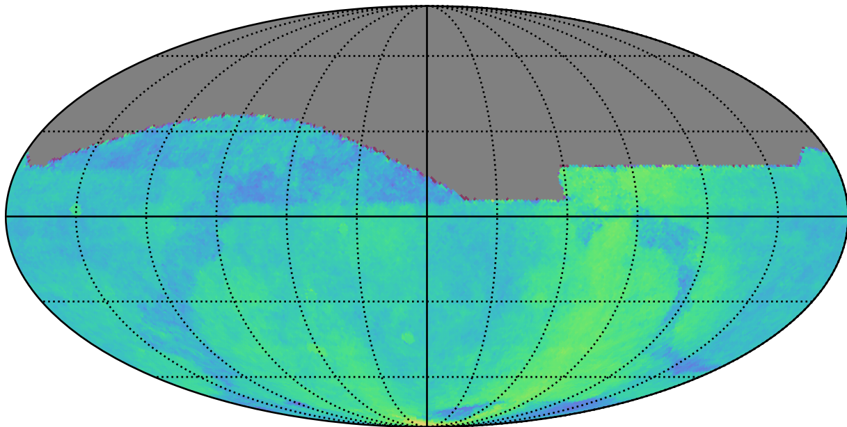
no_high_blob_v3.3_10yrs : Parallax Coverage @ 24.0
