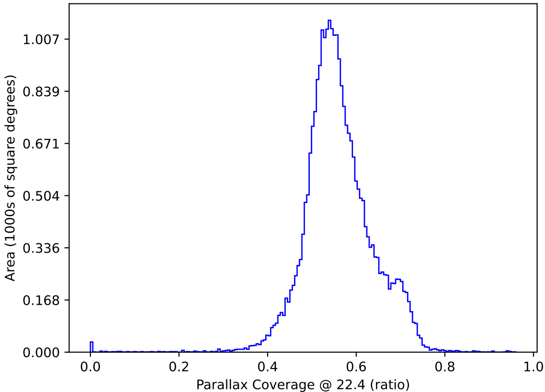
no_high_blob_v3.3_10yrs : Parallax Coverage @ 22.4
