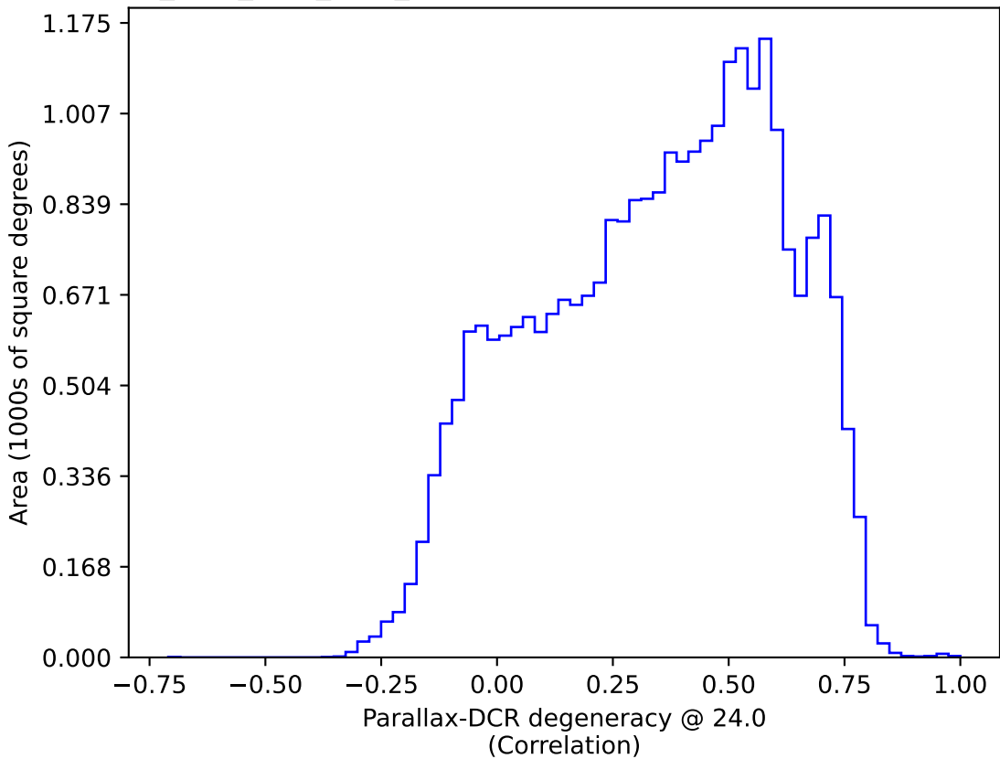
no_high_blob_v3.3_10yrs : Parallax-DCR degeneracy @ 24.0
