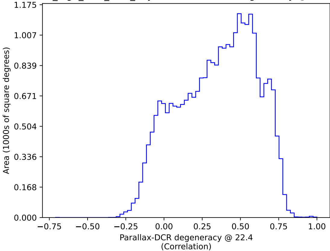
no_high_blob_v3.3_10yrs : Parallax-DCR degeneracy @ 22.4
