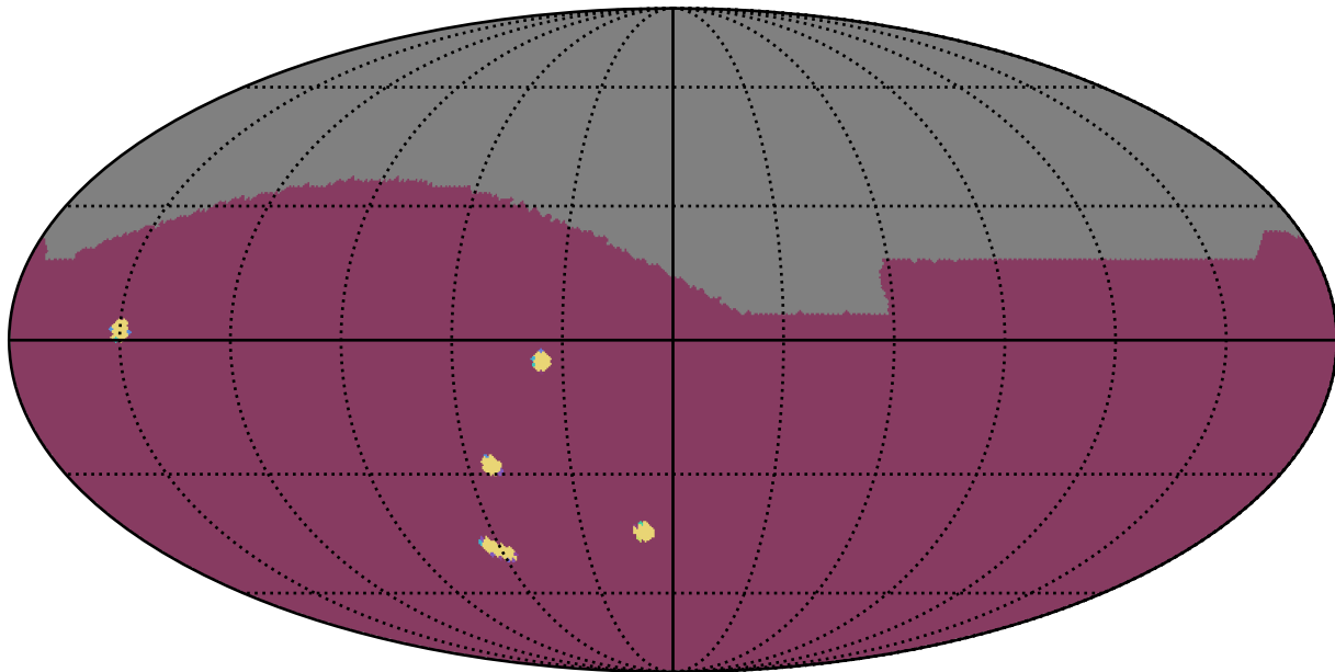
no_high_blob_v3.3_10yrs : NumberOfQuickRevisits
