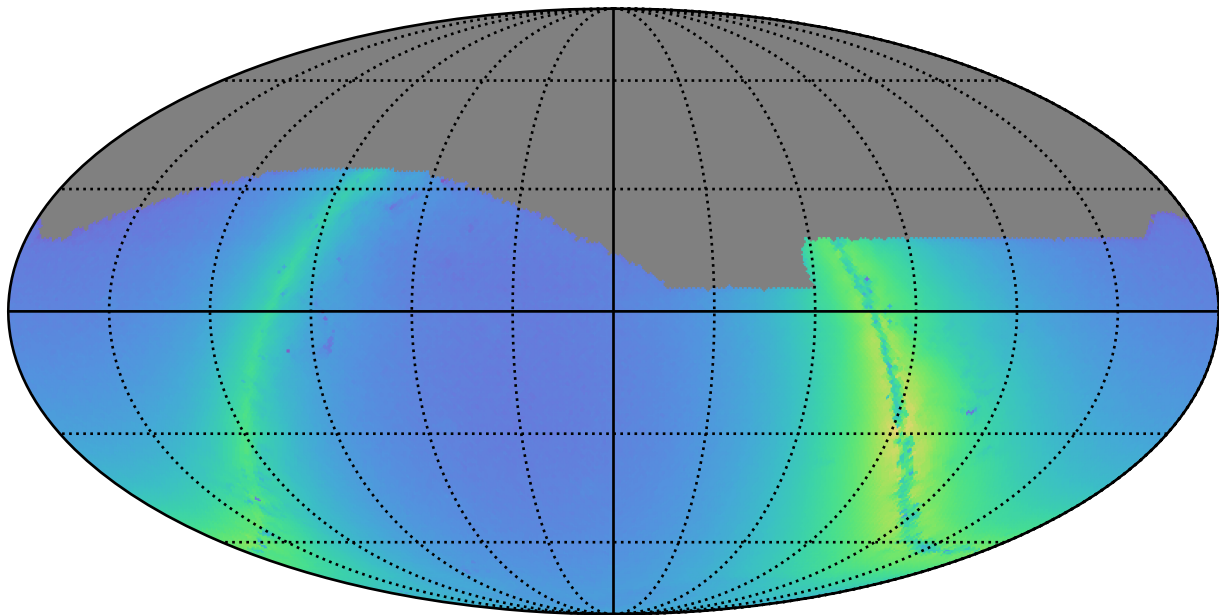
no_high_blob_v3.3_10yrs r: Nstars_no_crowding
