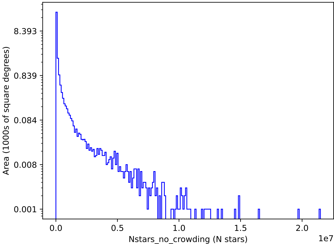
no_high_blob_v3.3_10yrs r: Nstars_no_crowding
