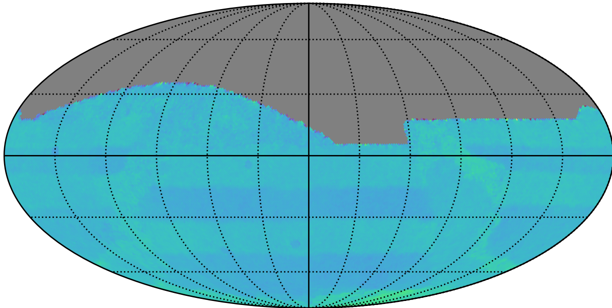
no_high_blob_v3.3_10yrs : Normalized Proper Motion Uncert @ 20.5
