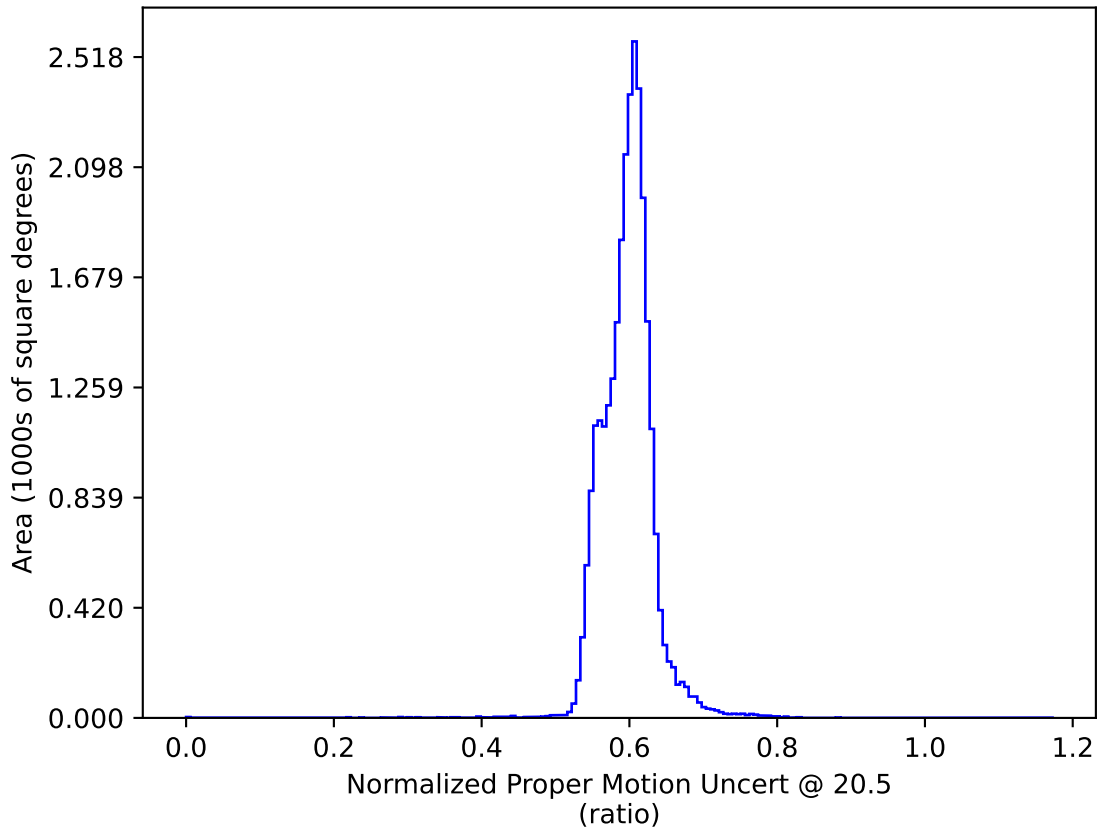
no_high_blob_v3.3_10yrs : Normalized Proper Motion Uncert @ 20.5
