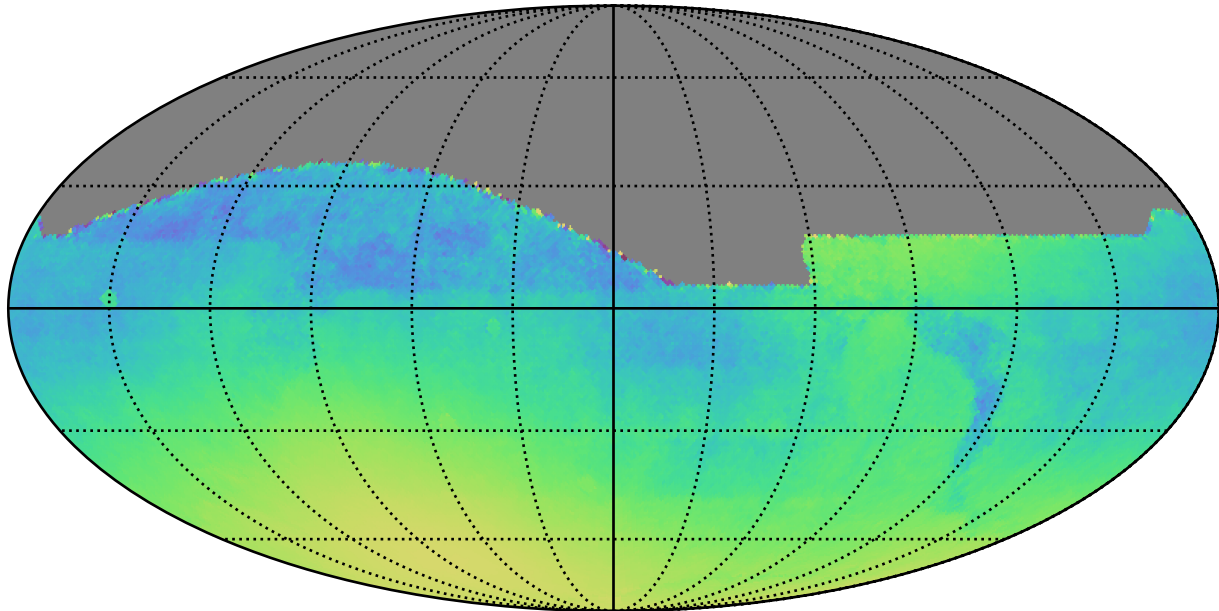
no_high_blob_v3.3_10yrs : Normalized Parallax Uncert @ 24.0
