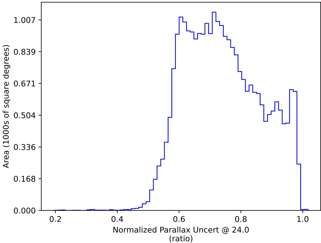
no_high_blob_v3.3_10yrs : Normalized Parallax Uncert @ 24.0
