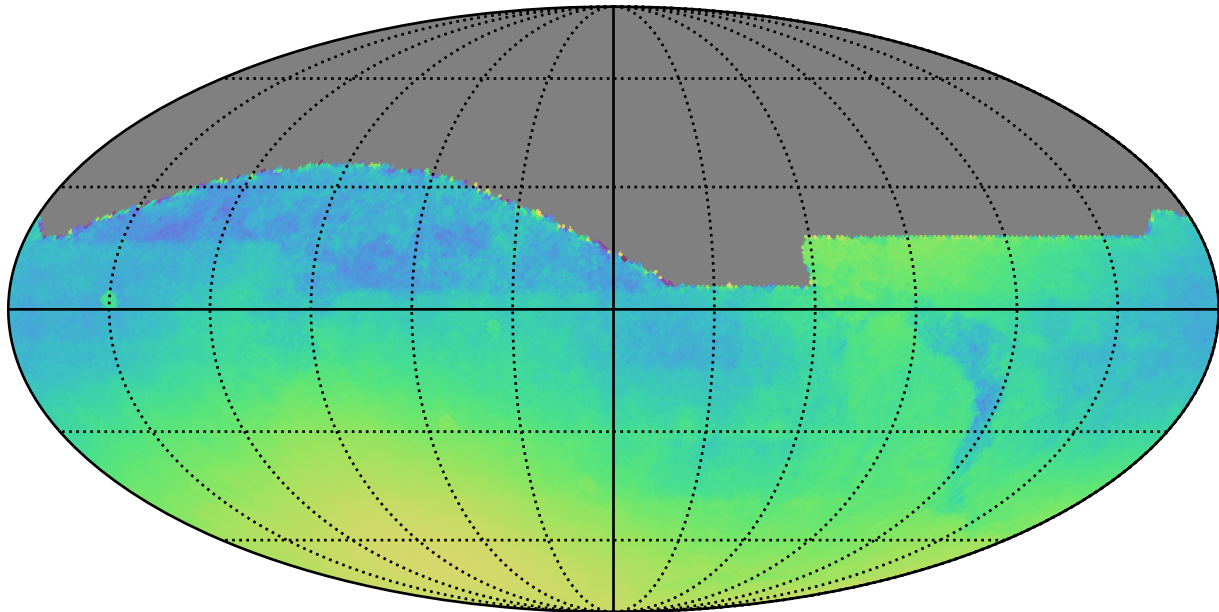
no_high_blob_v3.3_10yrs : Normalized Parallax Uncert @ 22.4
