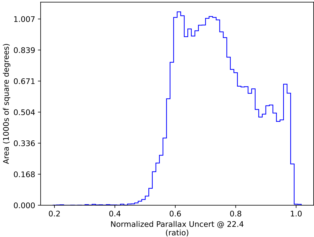
no_high_blob_v3.3_10yrs : Normalized Parallax Uncert @ 22.4
