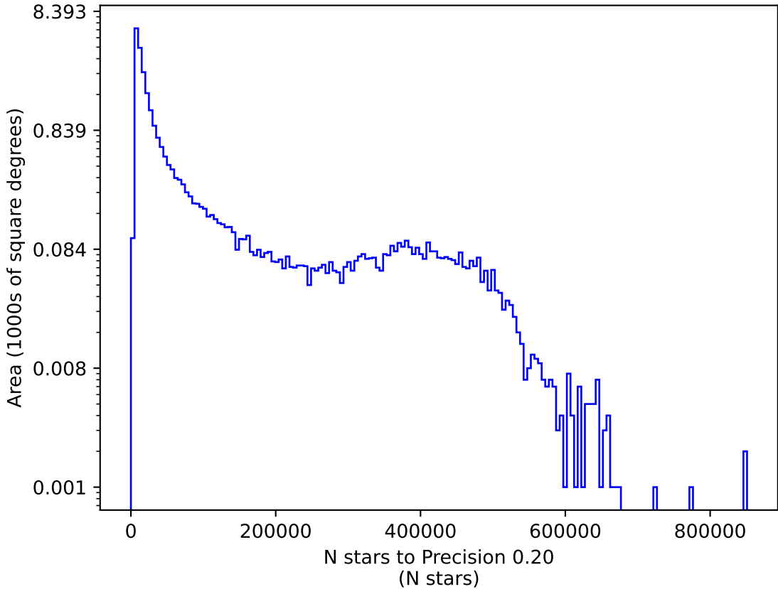
no_high_blob_v3.3_10yrs z: N stars to Precision 0.20
